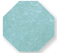
KI-27 Glacial Lake
